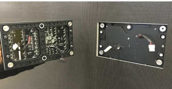
Wafer-thin, front service LED modules
